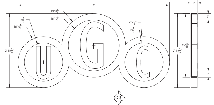
C-3 SECTION
